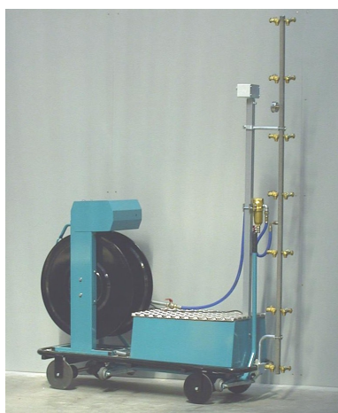
Spray trolley with hose reel, filter and spraying boom
